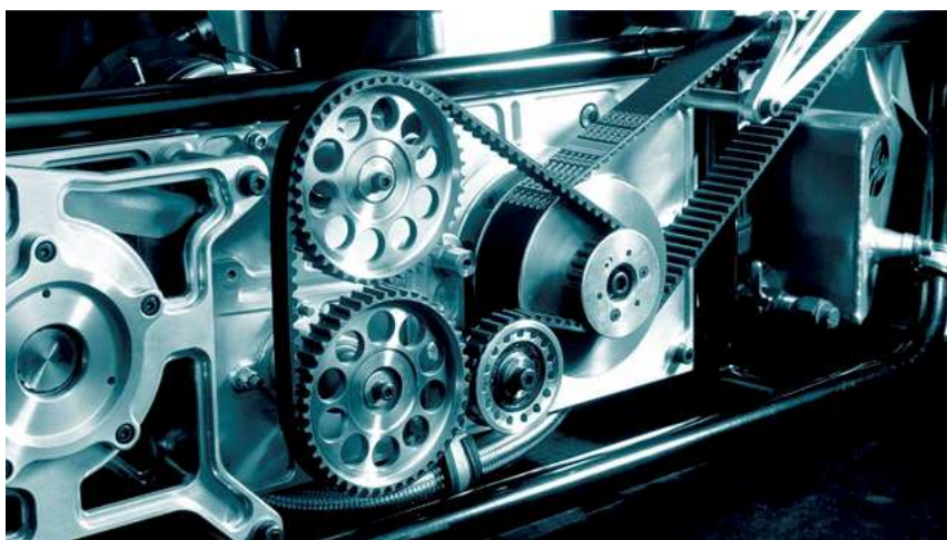
Therban - High performance elastomers for timing belts. (Photo ARLANXEO, ARPR001)
